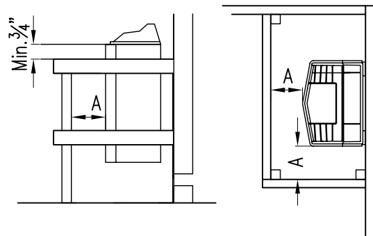
Minimum Distances for Heater Guard
